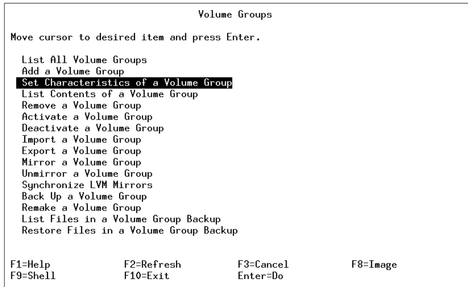
Figure 57. The Volume Groups Menu
