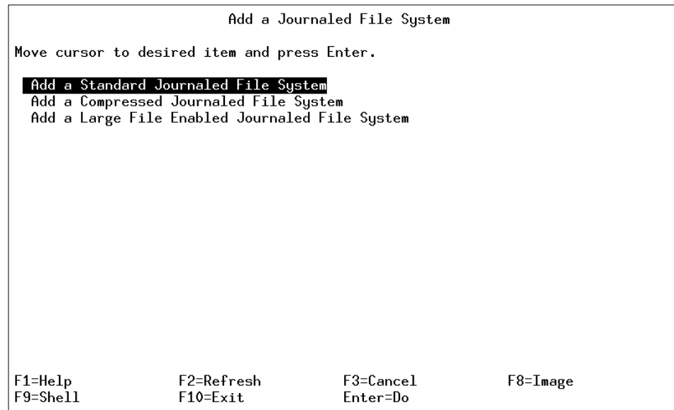
Figure 75. smitty crjfs - Step 1
